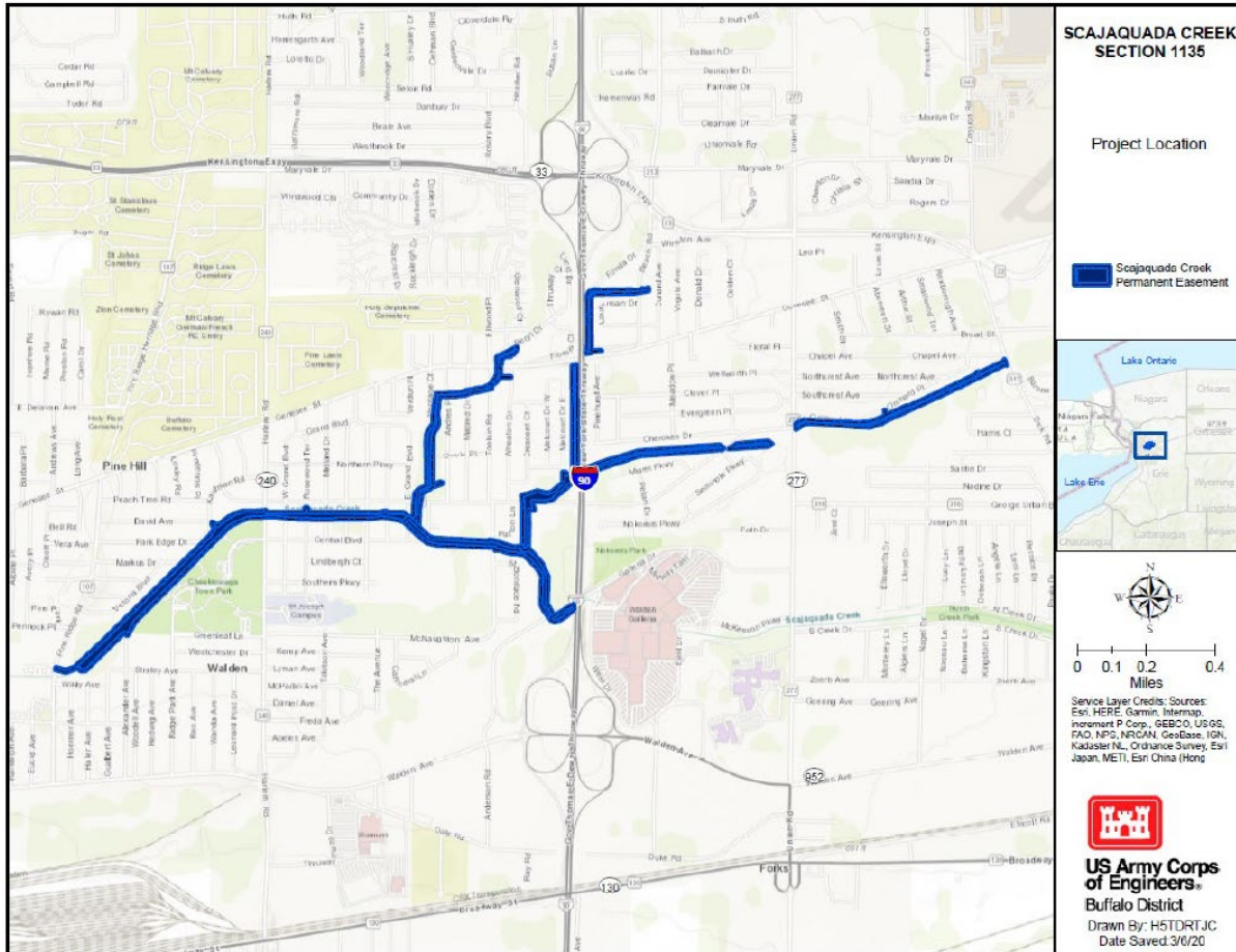
Figure 1. Limits of the USACE Scajaguada Creek Flood Risk Management Project, located within the Town of Cheektowaga, New York (Source: USACE).
