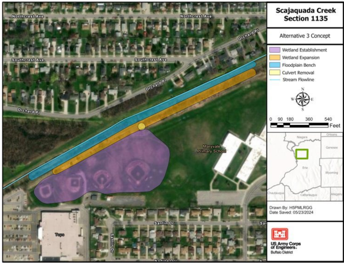
Figure 6. Alternative 3: Proposed site layout of the Maryvale Schools Ecosystem Restoration.
